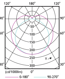
LEDtube MAS 14,7W G13 2300lm
